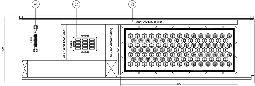
SECTION B-B RIO CABINET – XXXX
