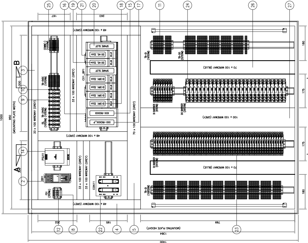
FRONT VIEW RIO CABINET – XXXX
