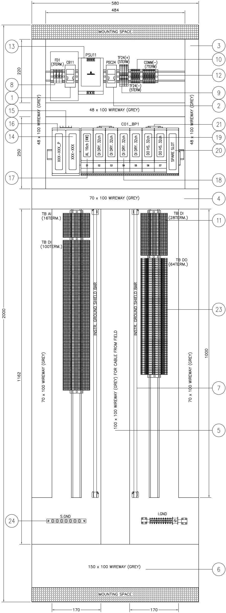
FRONT VIEW RIO MCC – XXXX
