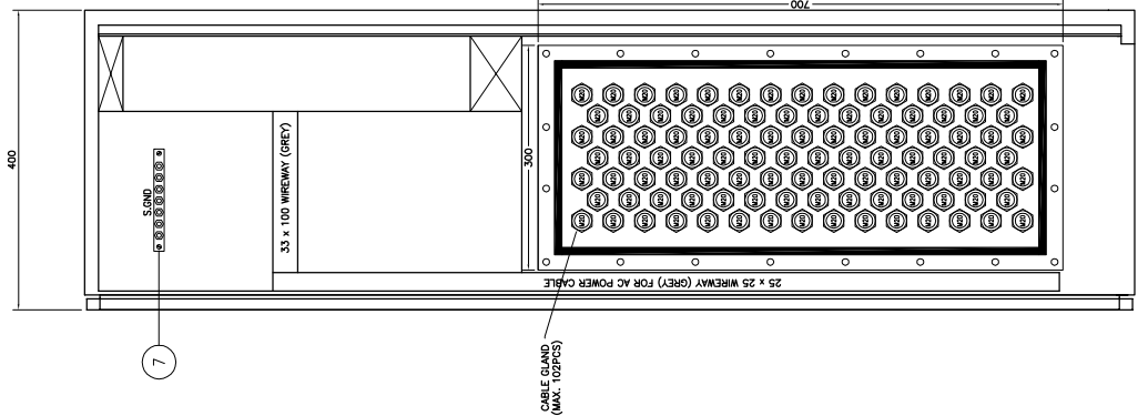
SECTION A-A RIO CABINET – XXXX
